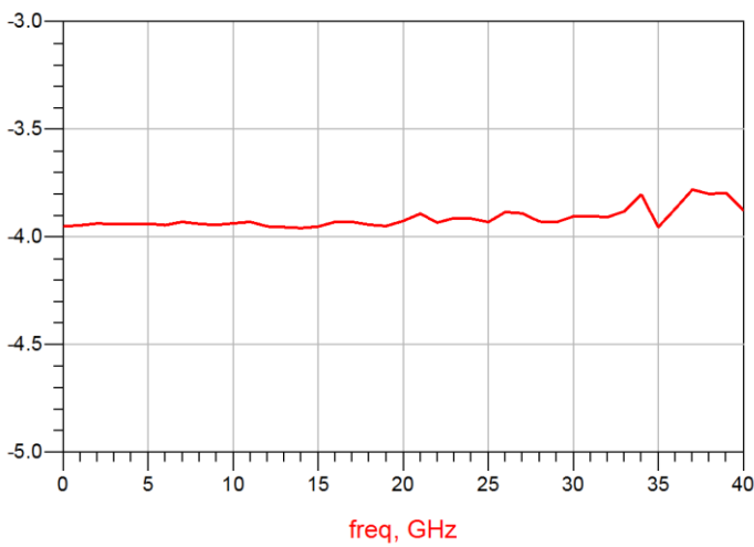
插入损耗
