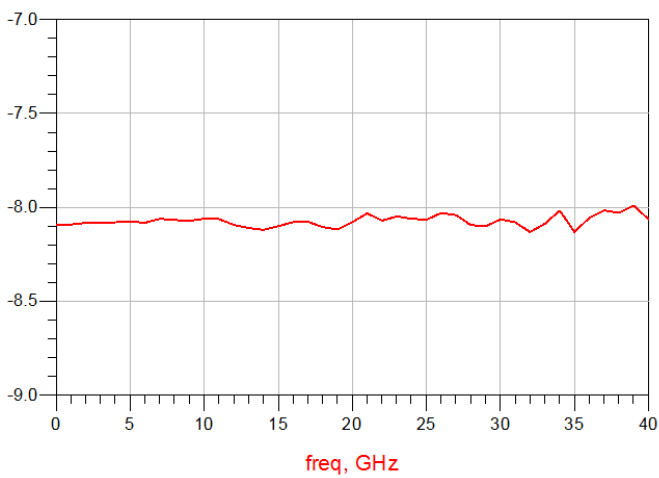
插入损耗
