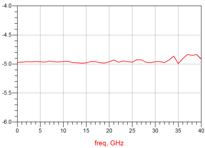
插入损耗
