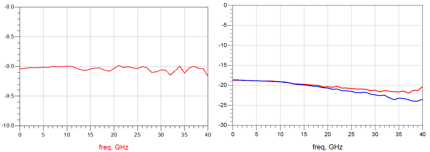
插入损耗
